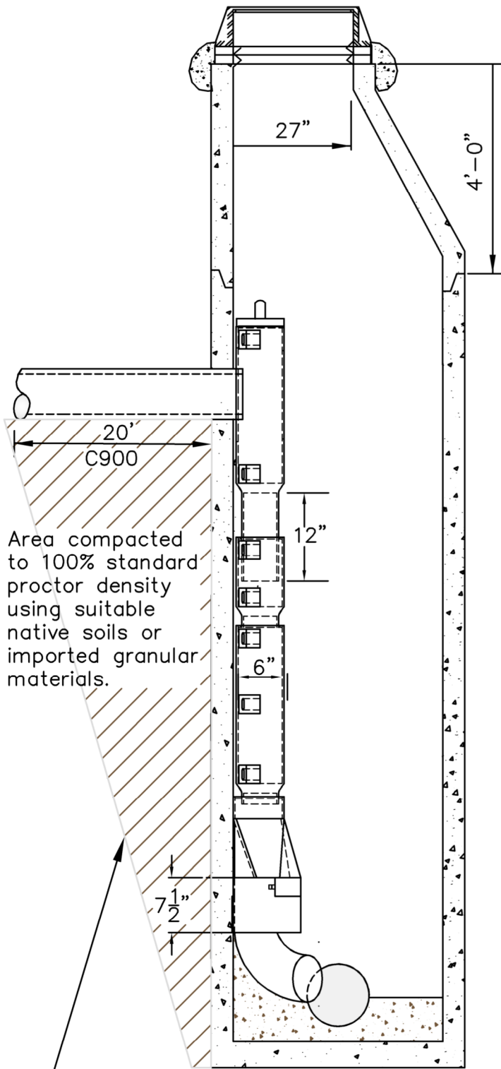
SECTION VIEW
