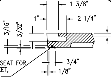
T-SEAL/CONCEALED PICKHOLE DETAIL GASKETED LIDS USED FOR SANITARY AND WATER MANHOLES
