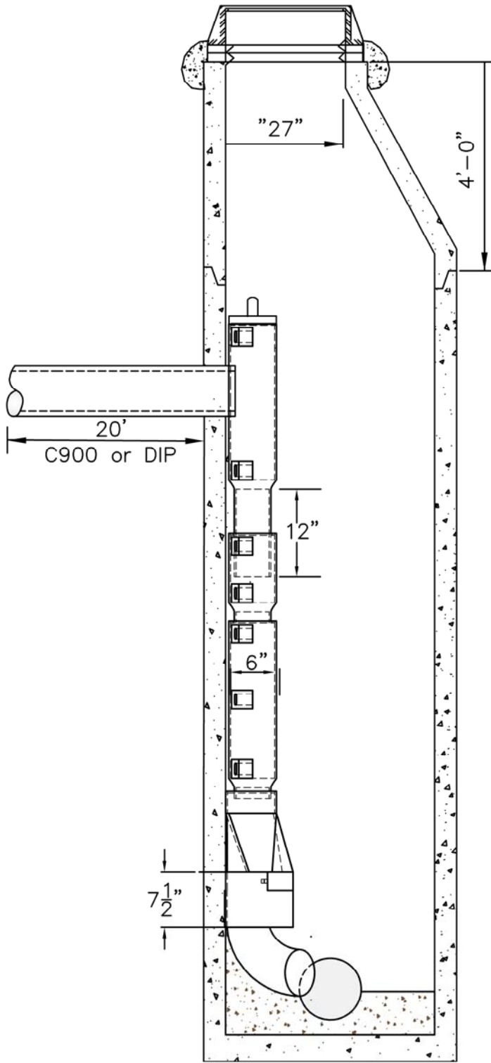
SECTION VIEW
