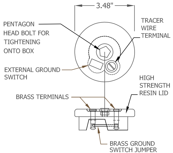
TWO-TERMINAL SWITCHABLE LID
